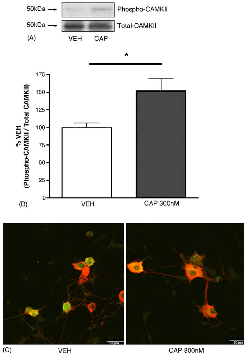
Fig. 2. TG neurons were exposed to VEH or 300 nM CAP for 10 min, scraped into tubes on ice and prepared for protein analysis by SDS-PAGE. Panel A illustrates a representative Western blot for phosho-CaMKII \alpha (Thr 286/287 ) and total CaMKII \alpha protein, which has been quantitated in panel B (* p < 0.05, Student's t -test). Panel C: Confocal images show independent TG neuronal culture representative photomicrographs taken at 63 \times (scale bar = 20 \mu m) of phospho-CaMKII \alpha immunoreactivity (green) and TRPV1-immunoreactivity (red, colocalization in yellow) in TG neurons exposed to VEH or CAP for 10 min.
