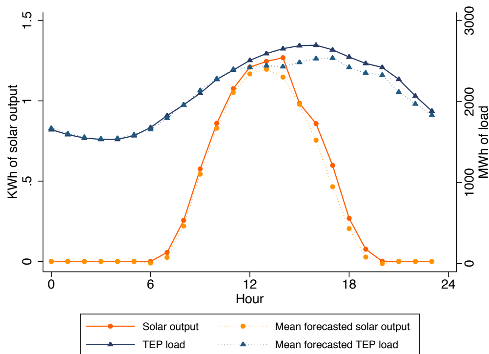
Figure 2: Predicted and actual southeastern Arizona load and solar output, Jul. 15, 2008
