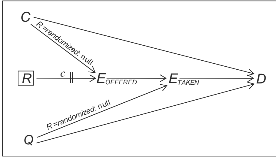
Fig. 4. Deconfounding by randomization ( R ), a modifier of the effects C \rightarrow E_{OFFERED} and Q \rightarrow E_{TAKEN} assuming that these effects are null when R= randomized (by some mechanism)
