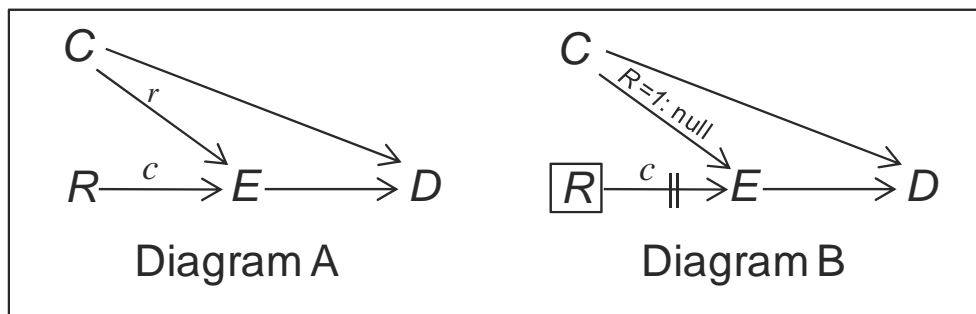
Fig. 3. Deconfounding by conditioning on R , a modifier of the effect C \rightarrow E (Diagram A), assuming that the effect C \rightarrow E is null when R=1 (Diagram B)
