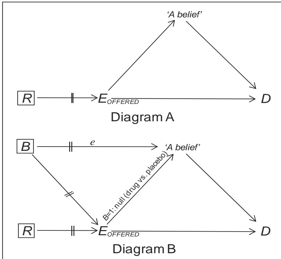
Fig. 16. The placebo path in a randomized trial (Diagram A); Removal of causal-pathway bias when we estimate the 'direct' effect E_{OFFERED} \rightarrow D (Diagram B)
