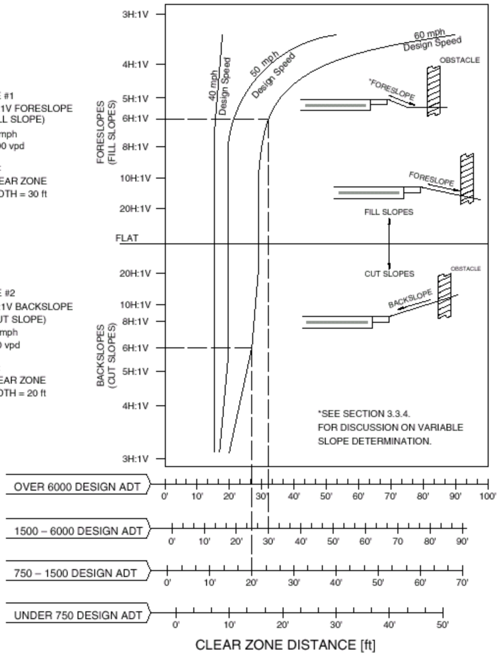
FIGURE 3.1b Clear-zone distance curves [U.S. customary units]
