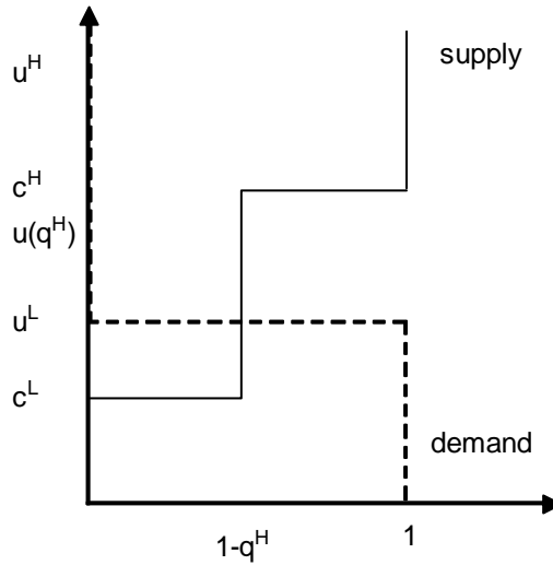
Figure 1(b): u(q^H) < c^H
