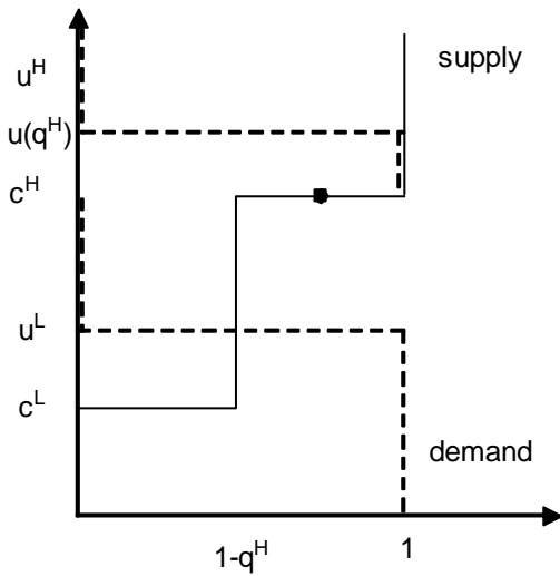
Figure 1(a): u(q^H) > c^H
