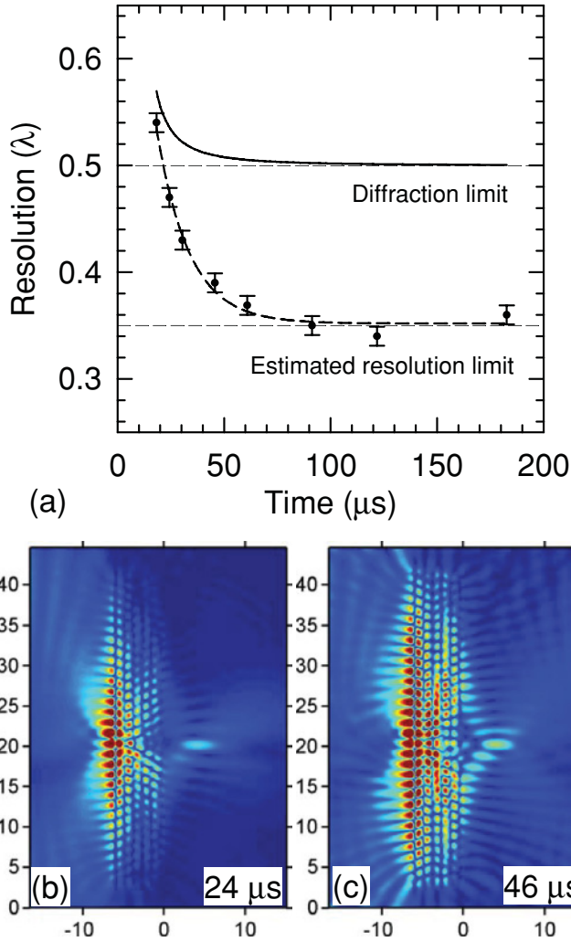
FIG. 9. (Color online) (a) Time evolution of the lateral resolution of the image in the standard configuration. The dashed line is an exponential fit to the data points, determined from FDTD simulations. The solid line is the lateral resolution of the half-width ( \Delta_p/2 ) as a function of time, as estimated using a simple ray tracing model involving only propagating modes (see text). (b) Pressure fields after 24 \mu\text{s} and (c) after 46 \mu\text{s} of propagation.
