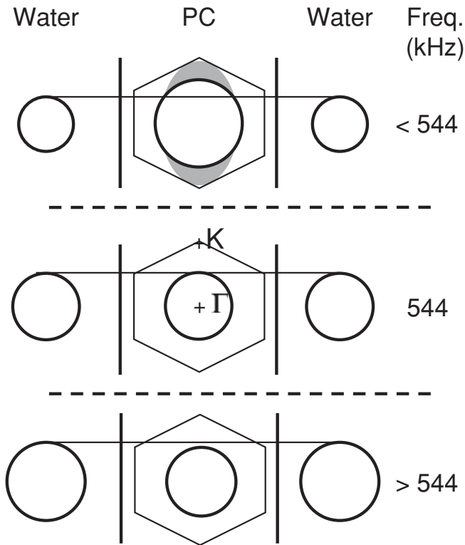
FIG. 5. Schematic representation of the transmission through the PC lens based on the equifrequency contours shapes. The equifrequency contour of the PC lens is represented as a circle inside the first Brillouin zone of the hexagonal infinite crystal. The gray areas illustrate the existence of bound modes with frequency very close to the operating frequency.
