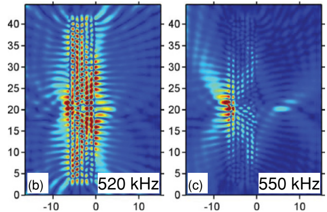
FIG. 4. (Color online) Effects of the operating frequency. (a) Lateral resolution and distance of the image as a function of the operating frequency. Results from experiments (triangles) are compared to FDTD simulation (circles). Pressure fields at 520 kHz (b) and 550 kHz (c).
