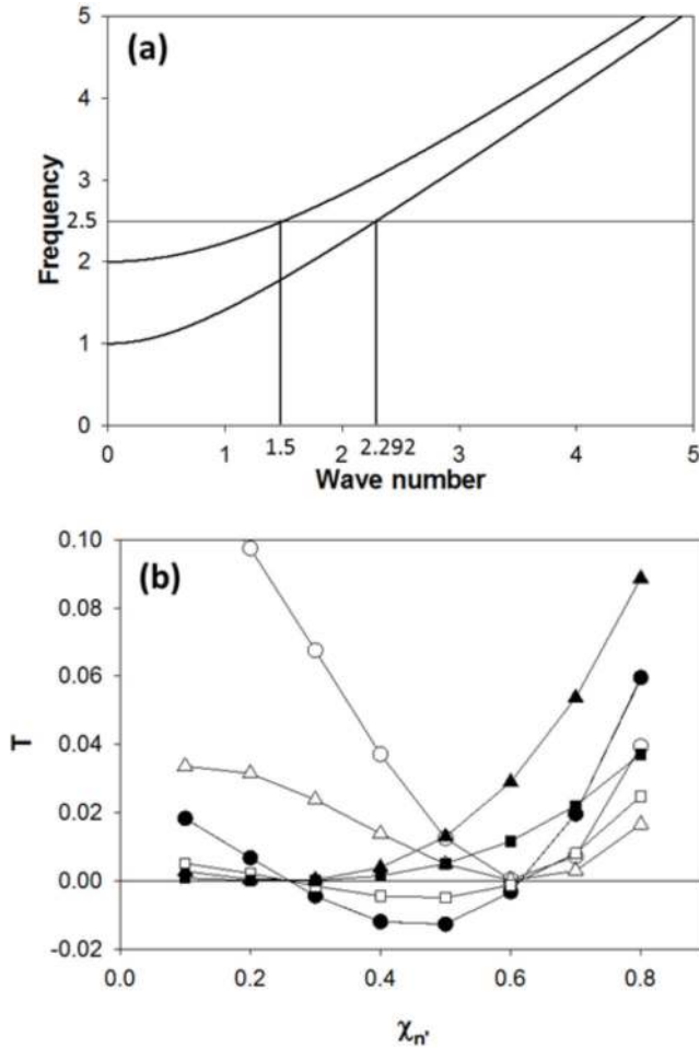
Figure 2. (a) Schematic illustration of the band structure for an array of three elastically coupled waveguides arranged in a ring pattern. Each of the waveguides is also grounded elastically to a rigid substrate. The upper band is doubly degenerate. We have taken \beta = 1 and \alpha = 1 . We highlight the frequency \omega_0 = 2.5 corresponding to the wave numbers k = 2.292 and k' = 1.5 . (b) Calculated values of T_1 (open circles), T_2 and T_3 (closed circles), T_4 (open triangles), T_5 (closed triangles), T_6 and T_7 (open squares) and T_8 (closed squares) as functions of \chi_n' for \chi_n = 0.4 . We have fixed x = 0 .
