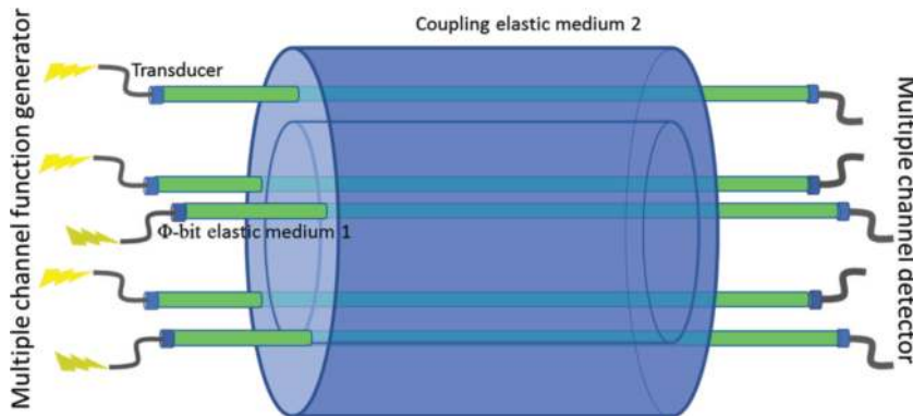
Figure 3. Schematic illustration of a five waveguide system. The waveguides are composed of an elastic medium 1 in which mass density and elastic stiffness determine the physical parameter \beta . The waveguides are embedded in an elastic medium 2 in which mass density and stiffness relate to the parameter \alpha . The waveguides are actuated via transducers (see the text for details).
