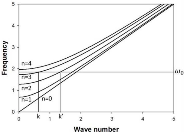
Figure 1. Schematic illustration of the band structure (circular frequency in \text{rad s}^{-1} versus the wave number in \text{m}^{-1} ) for an array of nine elastically coupled waveguides arranged in a ring pattern. The four upper bands are doubly degenerate. We have taken \beta = 1 and \alpha = 1 . The two modes with wave number k and k' ( n = 3 and n' = 2 ) have the same frequency \omega_0 .
