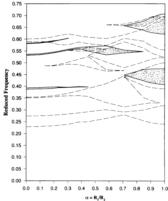
Figure 6. The variation of the width of the Z- (dashed lines) and XY- (solid lines) gaps appearing in the band structure of the BN arrays of epoxy cylinders in a carbon background, for f_1 + f_2 = 0.60 , as a function of the parameter \alpha = R_1/R_2 . The absolute band gaps are represented as speckled areas in this figure.
